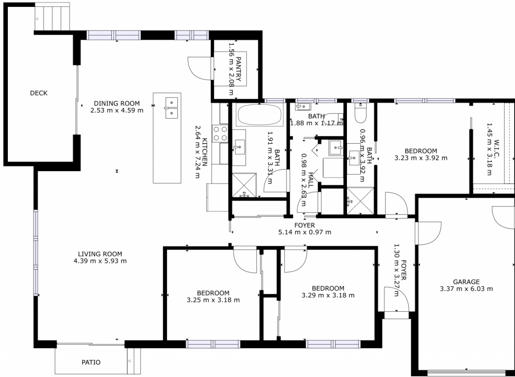
FLOOR 1
