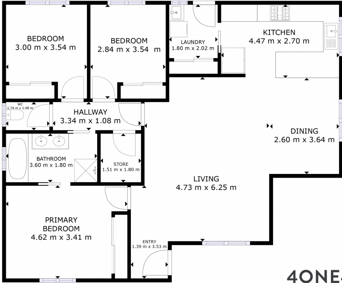
FLOOR PLAN
