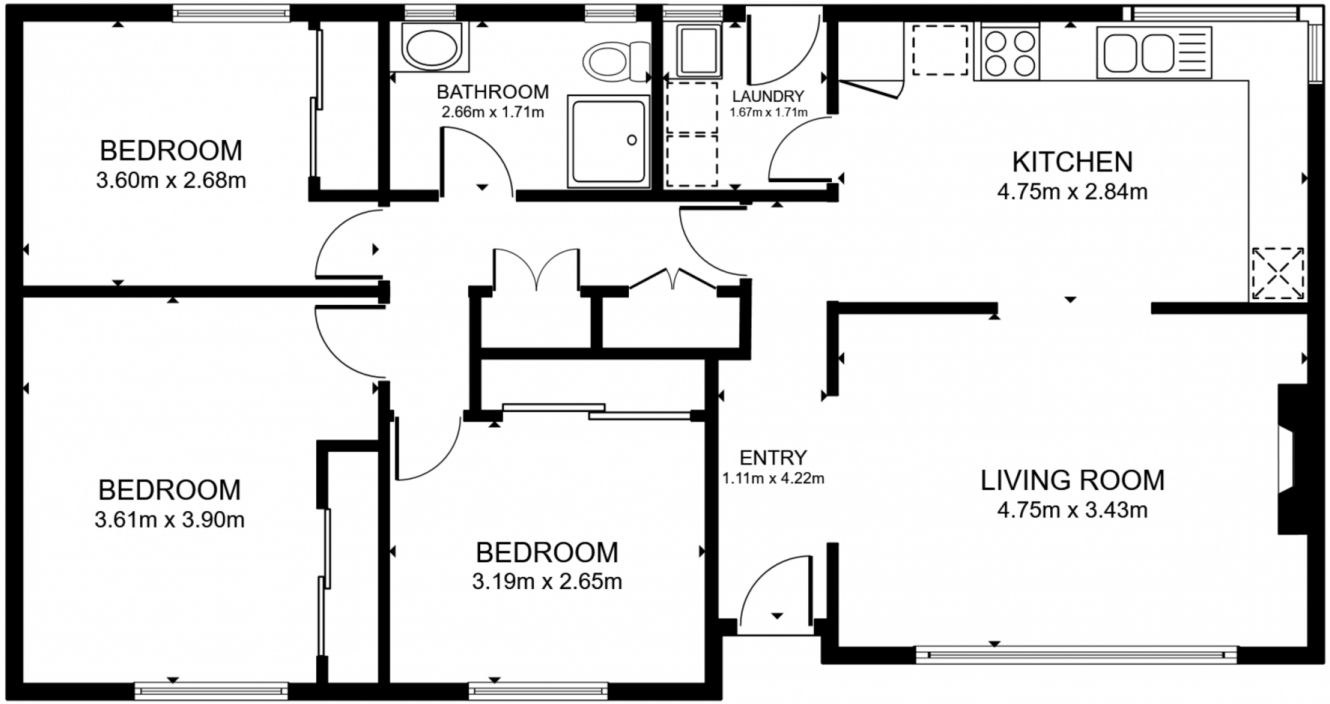
FLOOR PLAN FLOOR AREA 84.1 SQ.M. APPROX
