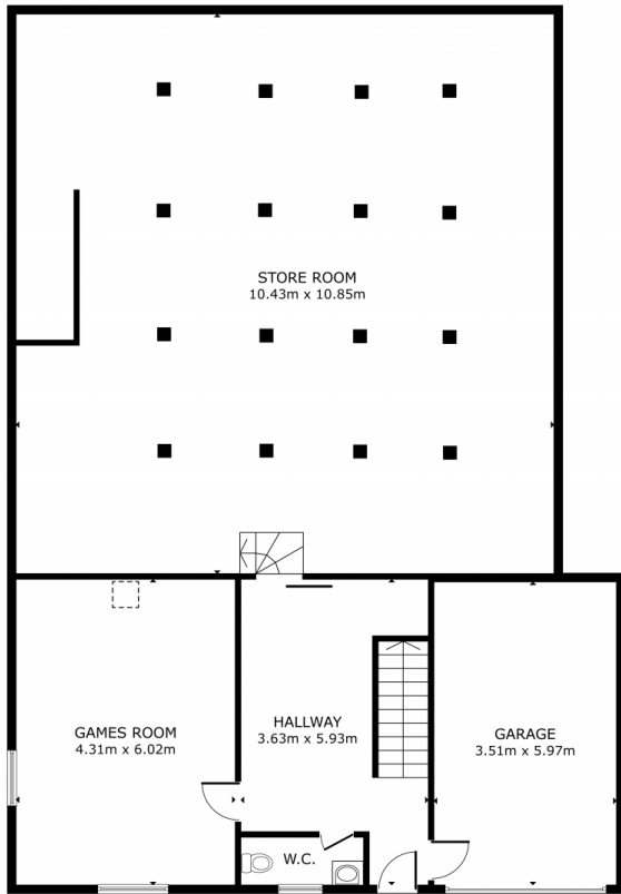
FLOOR 1
