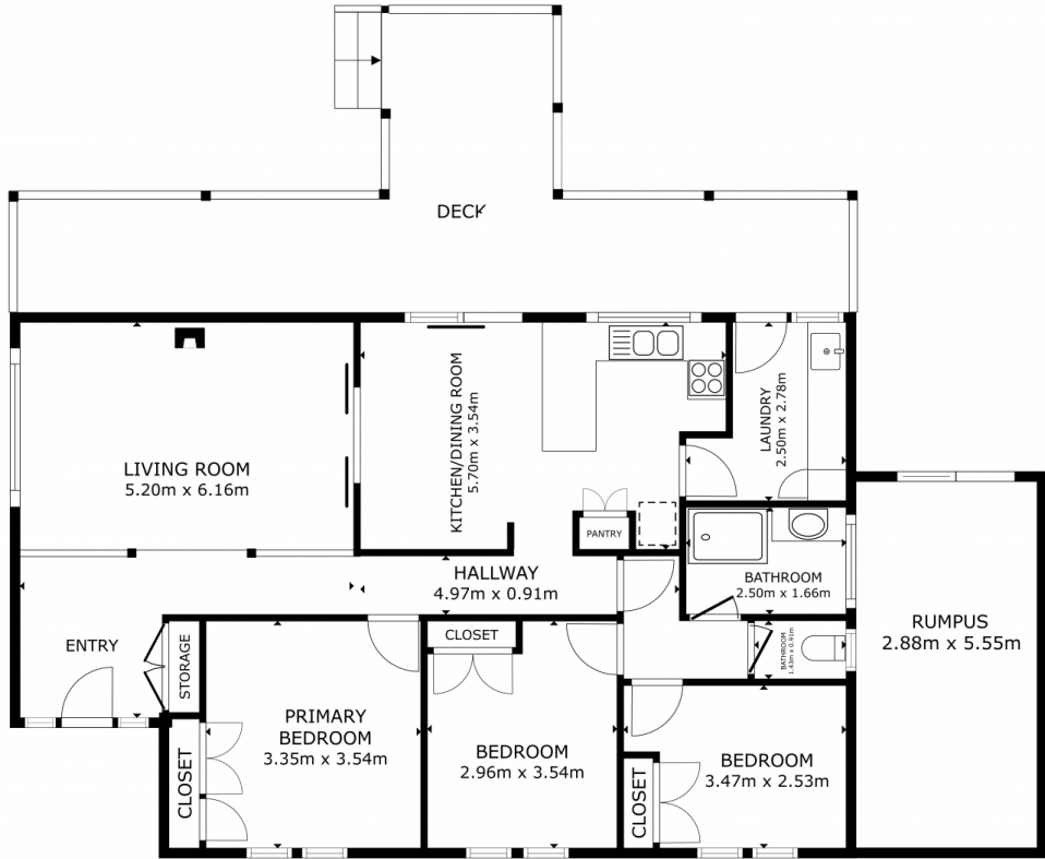
FLOOR PLAN
