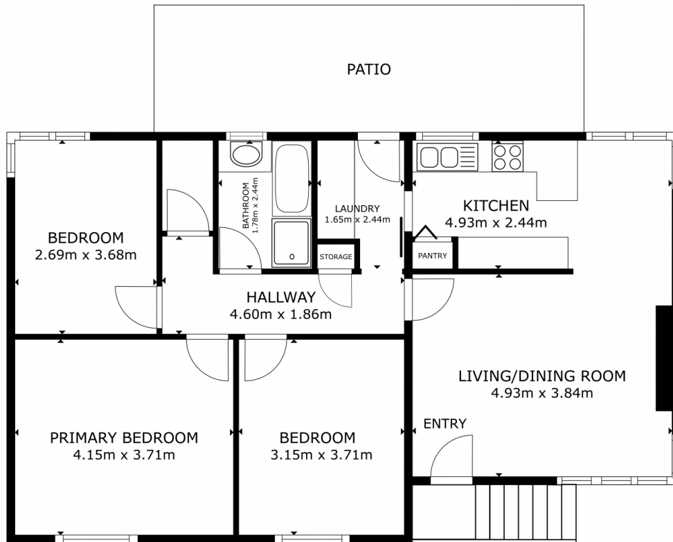
FLOOR PLAN
