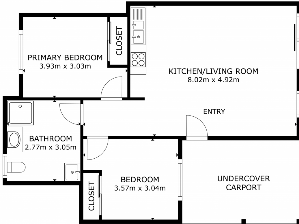
FLOOR PLAN
