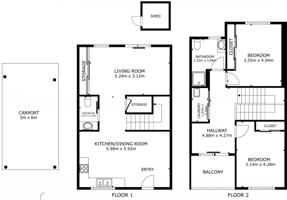
FLOOR 1
