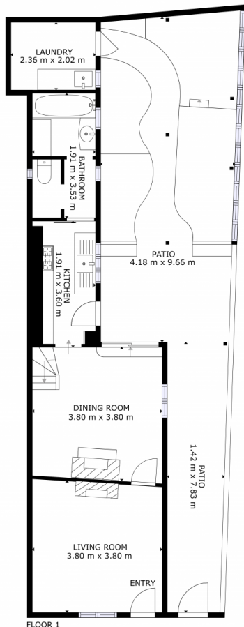
FLOOR 1
