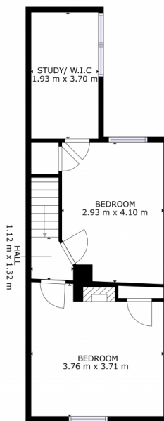
FLOOR 2
